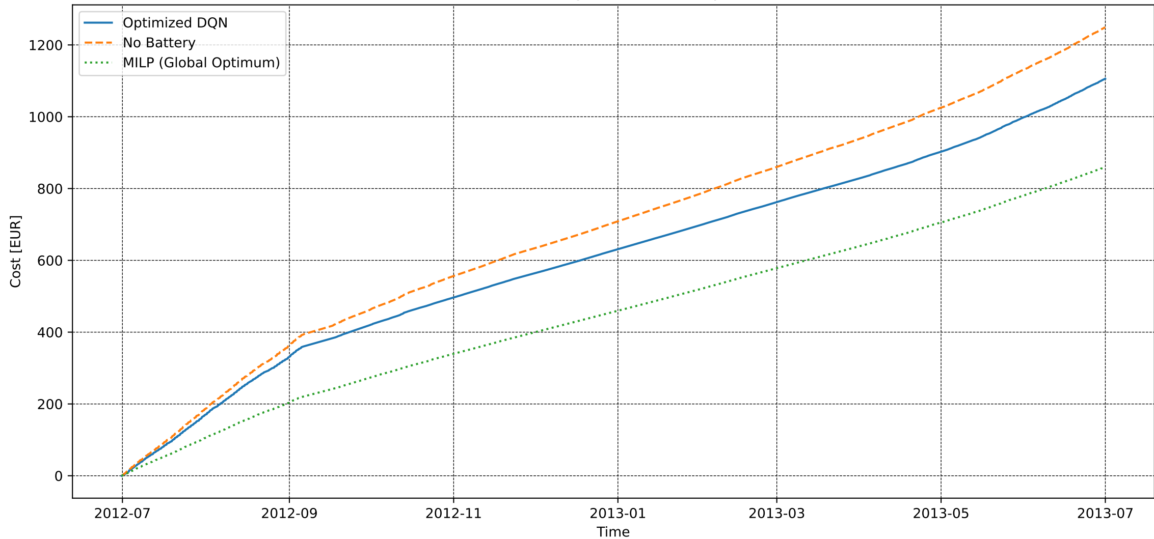
User 180 - Extended Convergence - Electricity Cost [DQN vs MILP]
